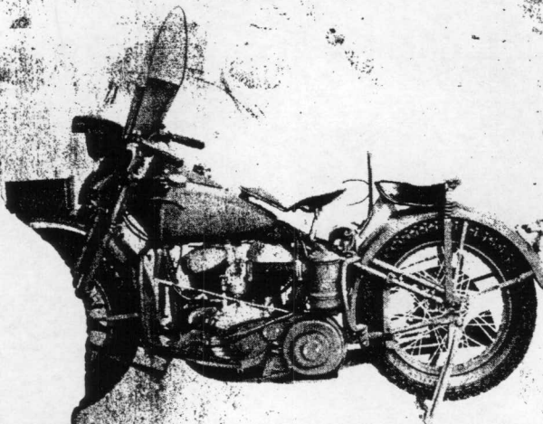
LEFT VIEW MODEL 1943 WLC MOTORCYCLE (EXPORT)
