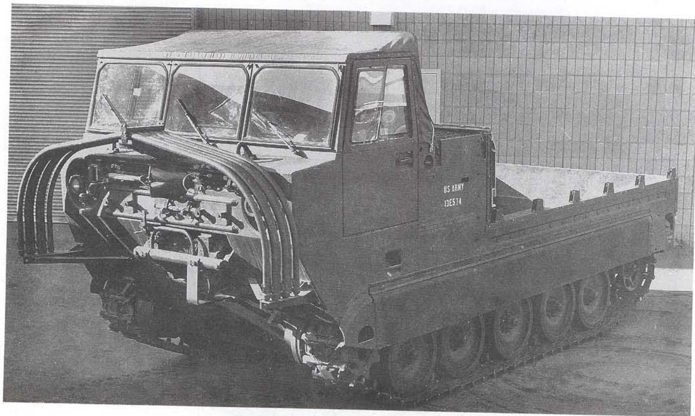
Figure 1-13. M730A2 Guided Missile Equipment Carrier.
