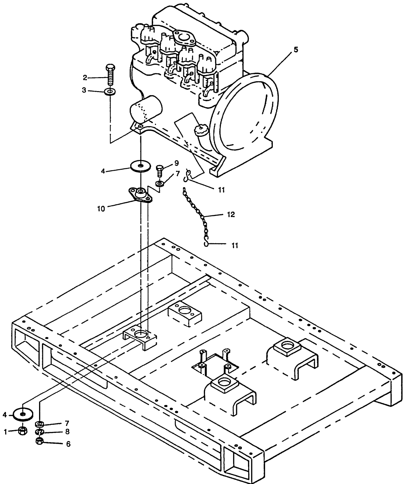
Figure 26. Engine Installation
