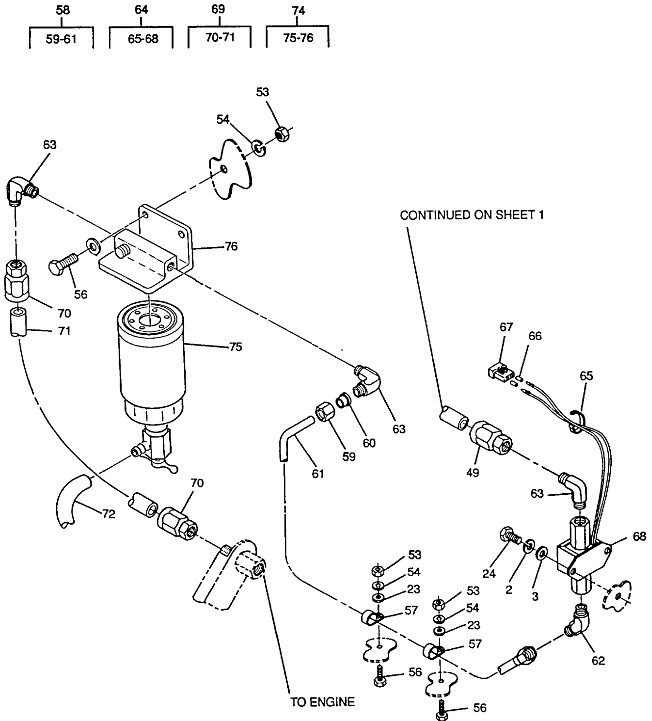
Figure 17. Fuel Tank Pumps and Lines (Sheet 2 of 2)
