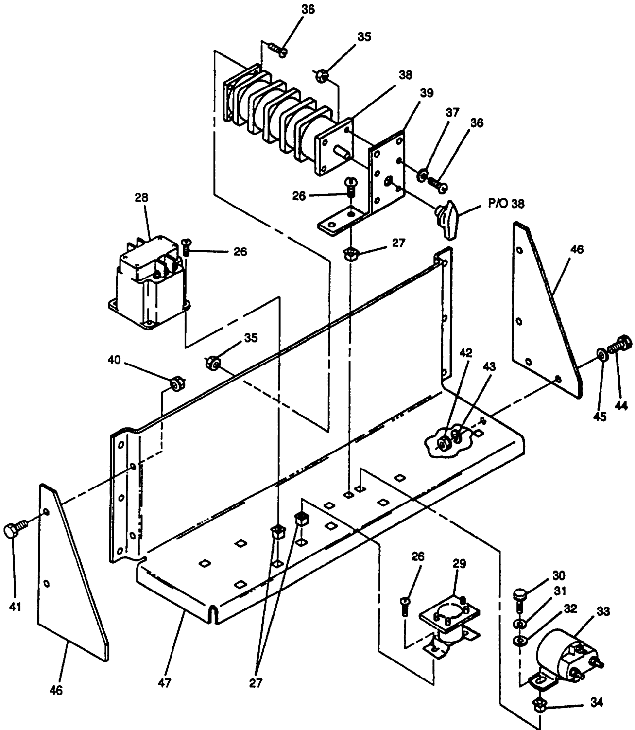
Figure 13. Output Box Components (Sheet 2 of 2)
