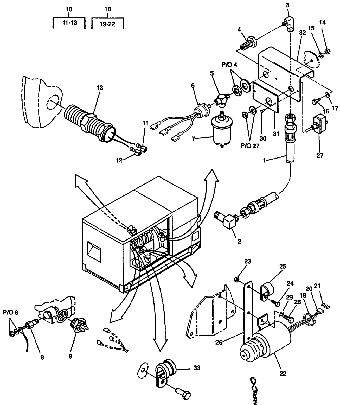
Figure 20. Engine Accessories
