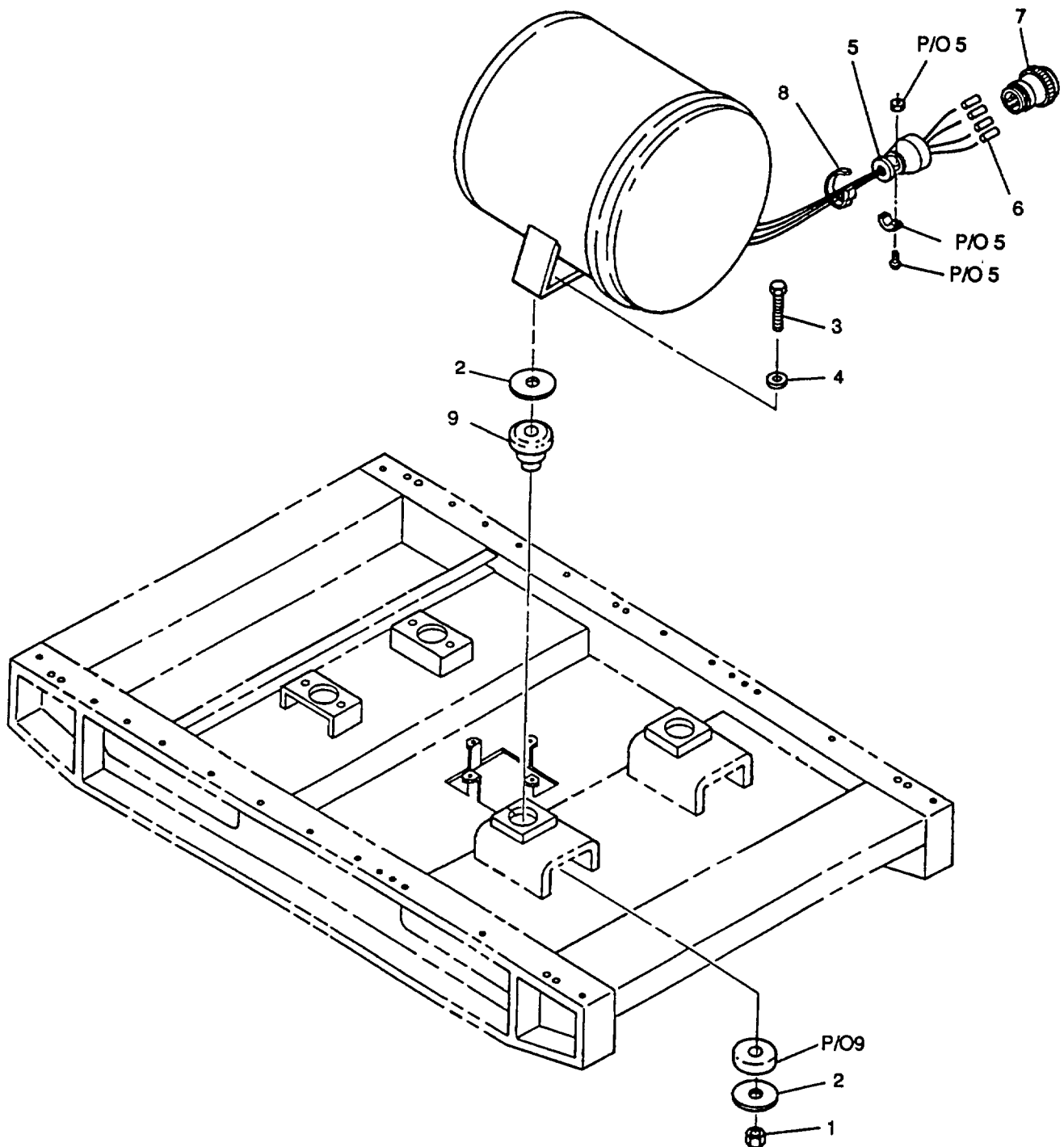
Figure 23. Generator Installation
